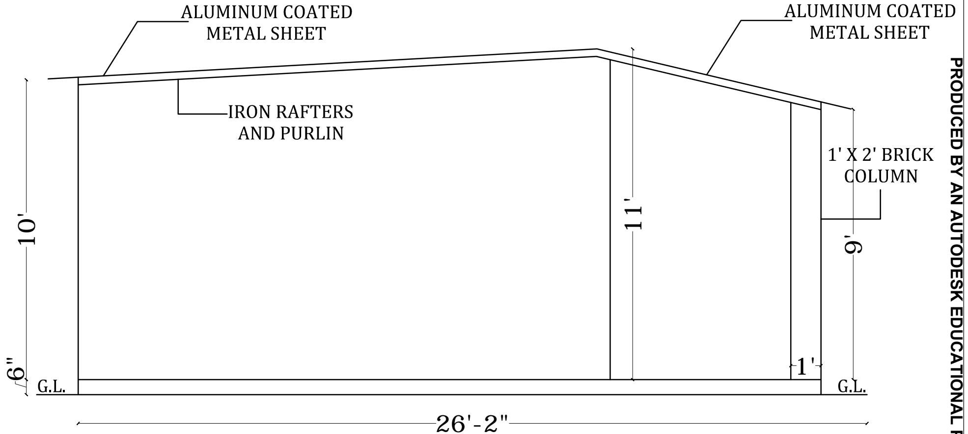
SIDE ELEVATION
